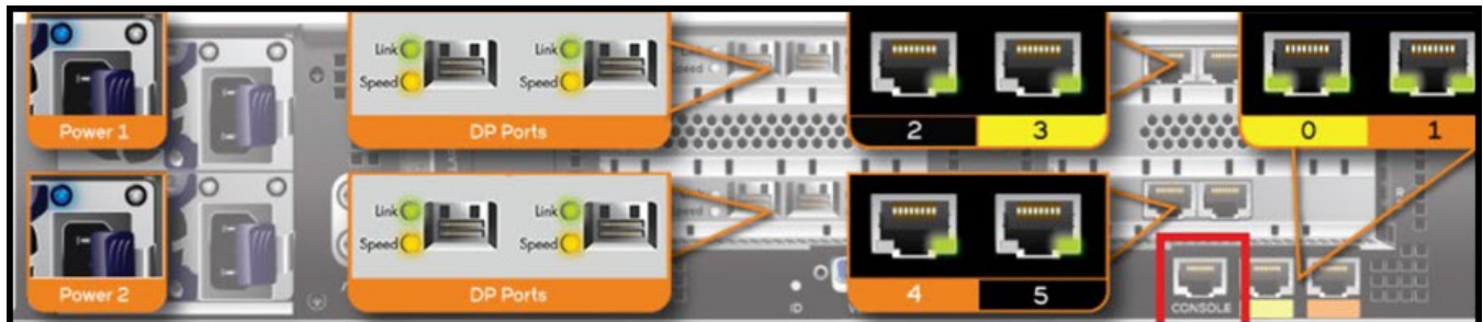
FIGURE 2 SZ300 Location of console port
